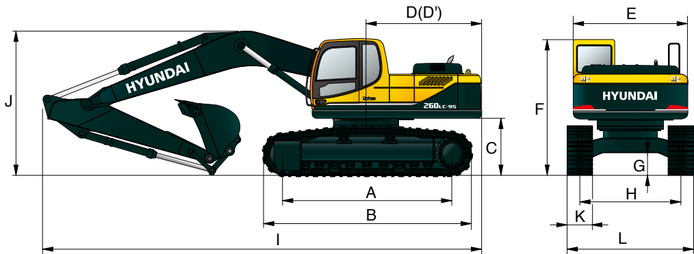
R260LC-9S HIGH WALKER DIMENSIONS
