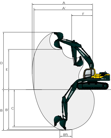
R260LC-9S HIGH WALKER WORKING RANGE
